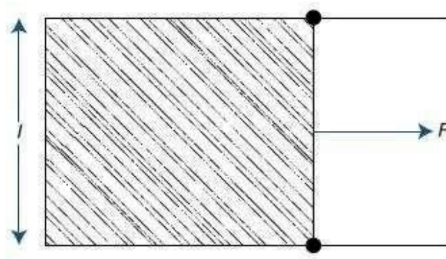
Fig. 1: A movable wire frame containing a film of liquid being expanded with a force F
