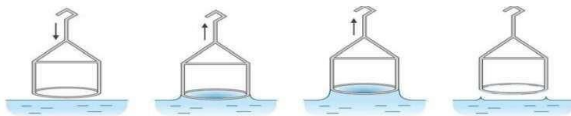
Fig. 3: Schematic of the DuNouy ring pulling a column of water above the surface
